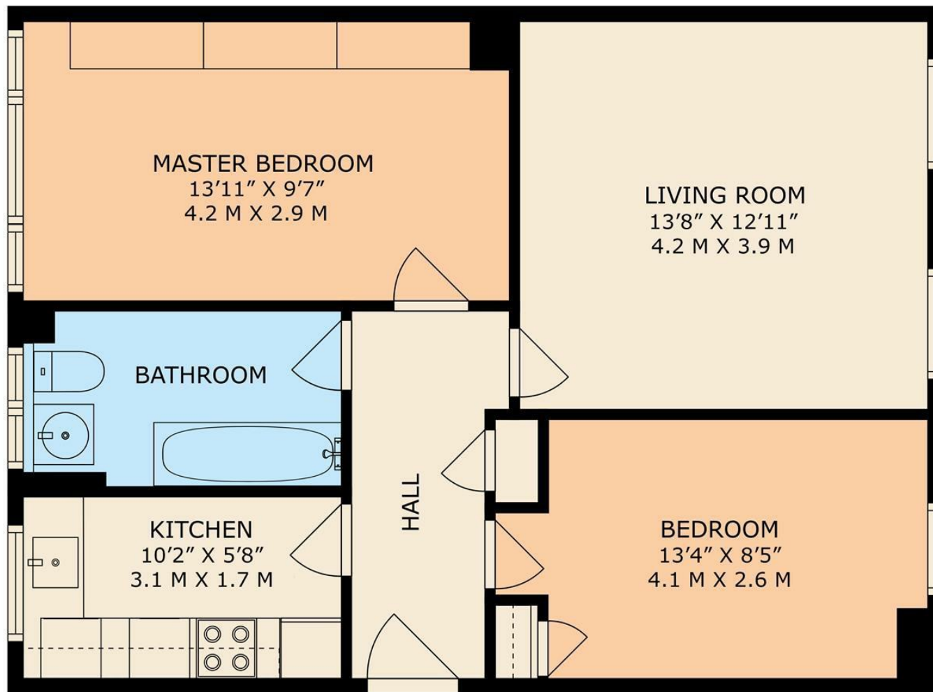
FIRST FLOOR
